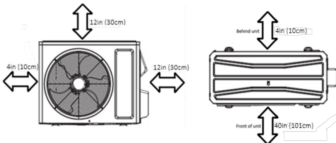
Minimum outdoor unit clearances
